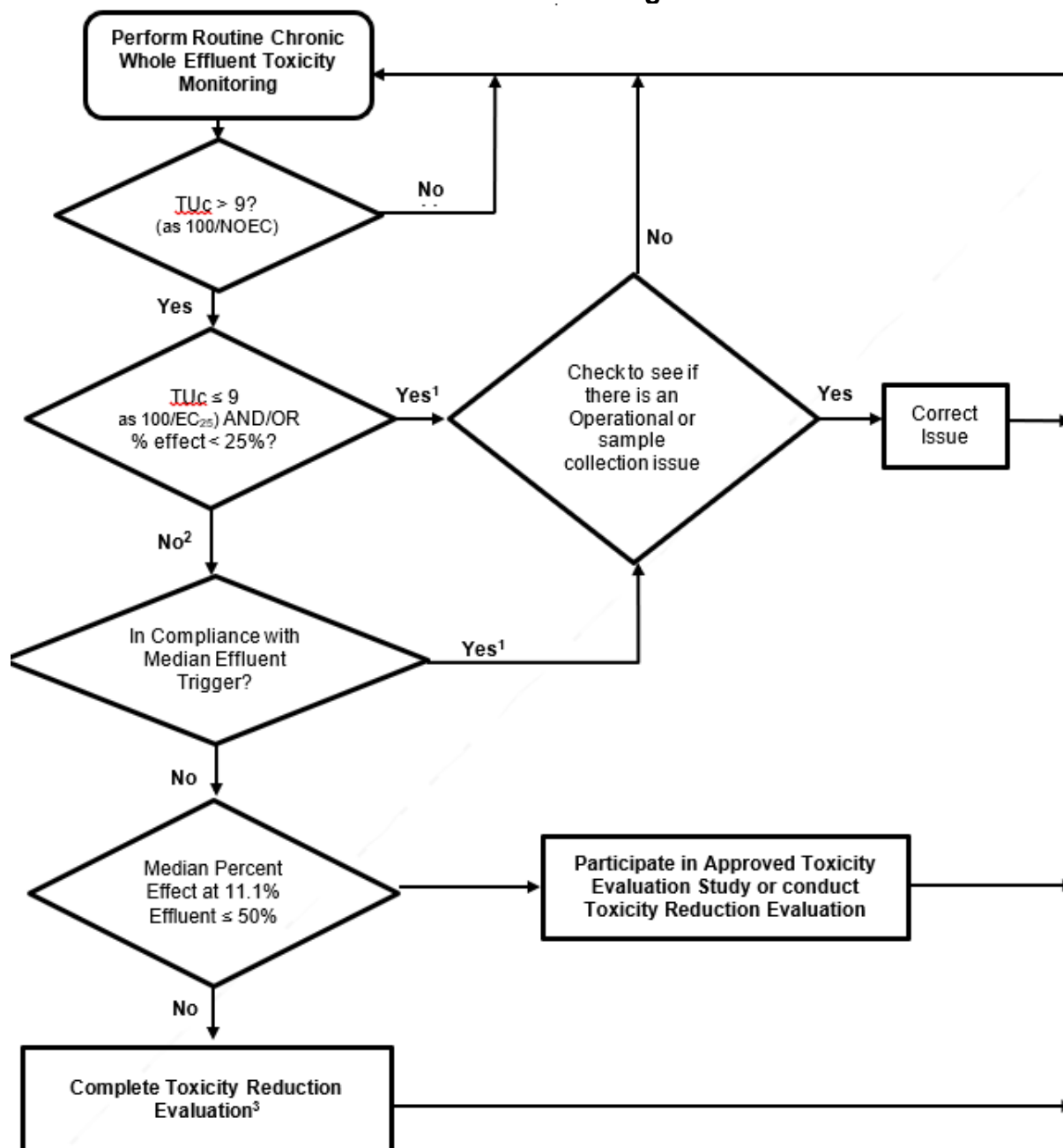
Figure F-2. WET Accelerated Monitoring Flow Chart
